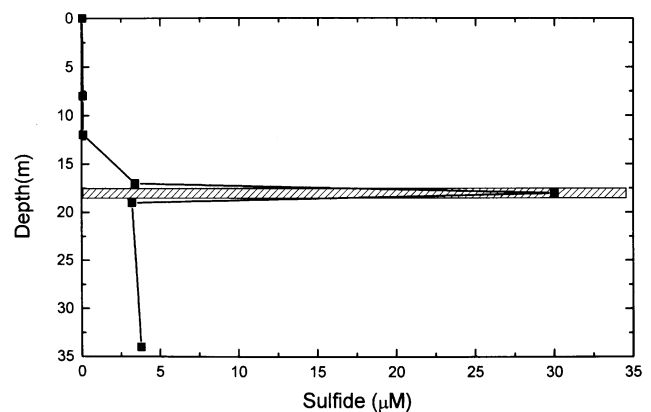
Fig. 6. Free sulphide profile of the South Andros Black Hole and position of the dense microbial layer in the water column determined in the early afternoon on 27 June 1999. Hatched area shows the position of the metre thick bacterial layer in the water column.
