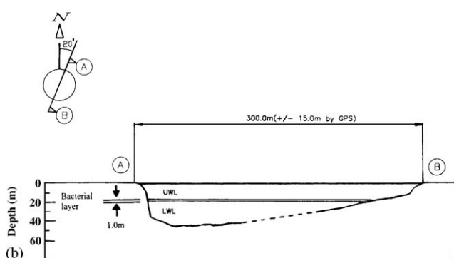
Fig. 2. Appearance of the South Andros Black Hole, (a) aerial view and (b) bathymetry. UWL, upper water layer; LWL, lower water layer; — floor area not surveyed.
