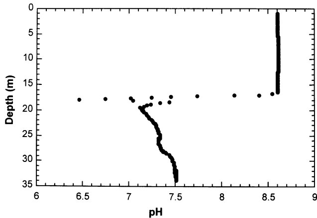
Fig. 7. The pH profile of the South Andros Black Hole measured in the early afternoon on 27 June 1999.
