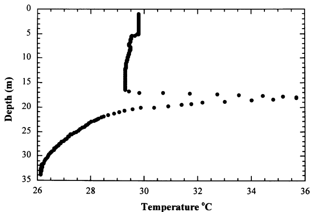
Fig. 4. Temperature profile of the South Andros Black Hole measured in the early afternoon on 27 June 1999.
