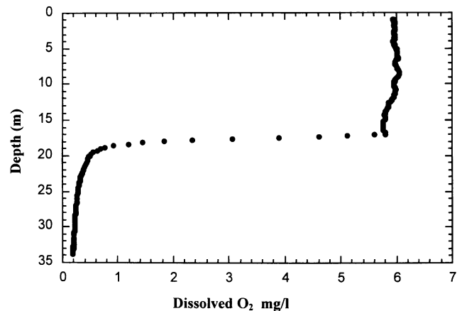
Fig. 5. Dissolved oxygen profile of the South Andros Black Hole measured in the early afternoon on 27 June 1999.
