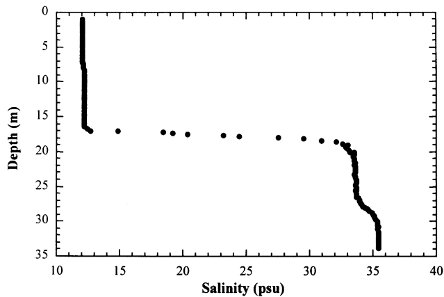
Fig. 3. Salinity profile of the South Andros Black Hole measured in the early afternoon on 27 June 1999.
